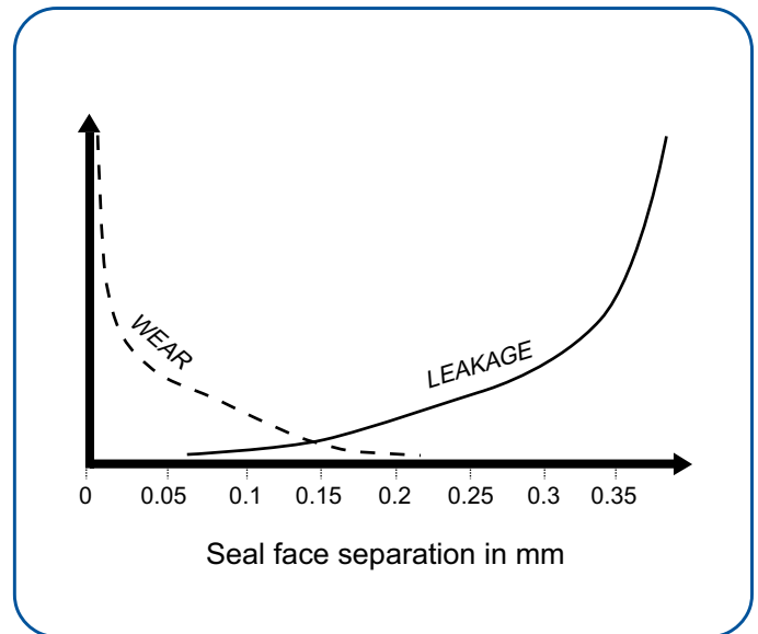
FIGURE 2: Leakage and wear rate vs face separation
