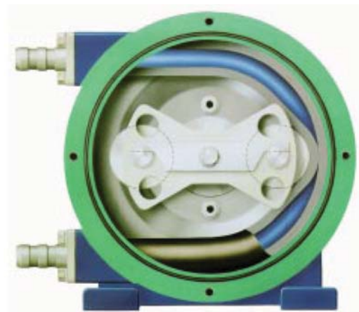
Figure 6: Peristaltic (hose or flexible tube) pump
