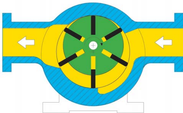
Figure 12: Positive displacement rotary vane pump
