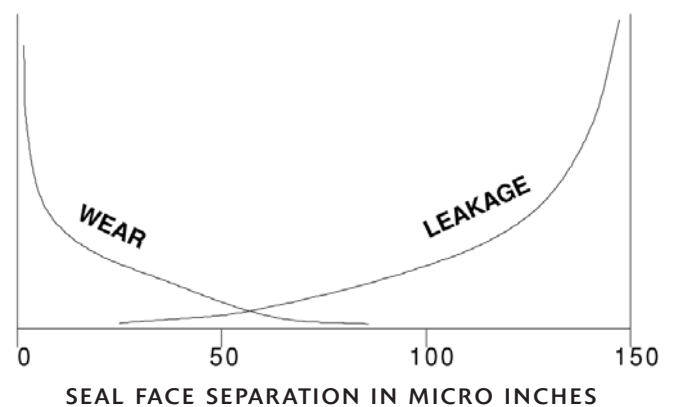
Figure 2: Mechanical seal leakage vs. life
