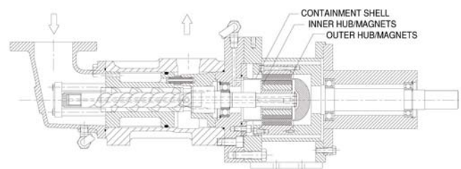
Figure 13: Magnetic drive three screw pump
