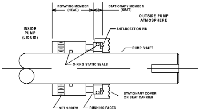
Figure 1: Conventional mechanical seal
