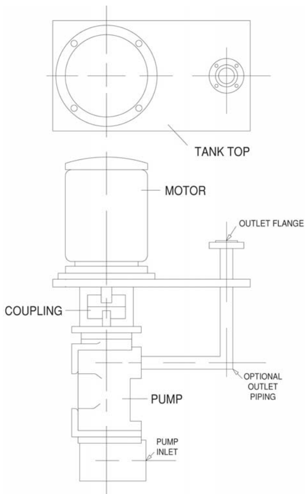
Figure 4: Unsealed tank mount main and emergency lube pumps
