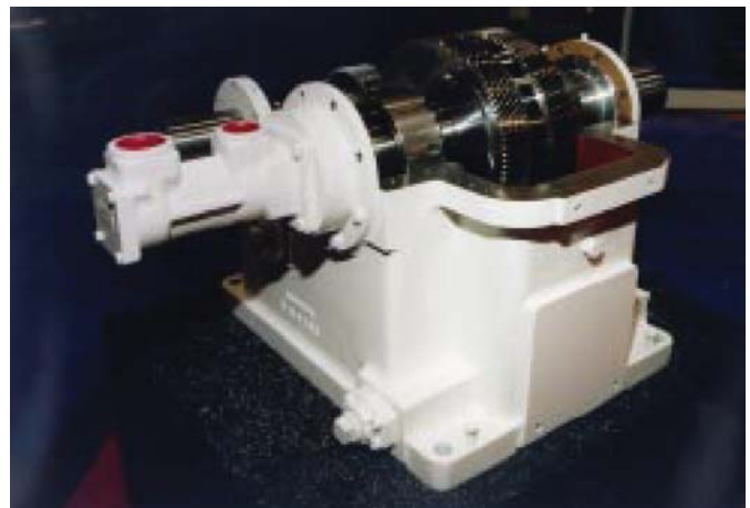
Figure 5: Unsealed lube pump driven by lubricated machine
