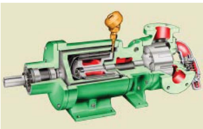
Figure 9: Magnetic drive internal gear pump with temperature probe (Courtesy Viking Pump)
