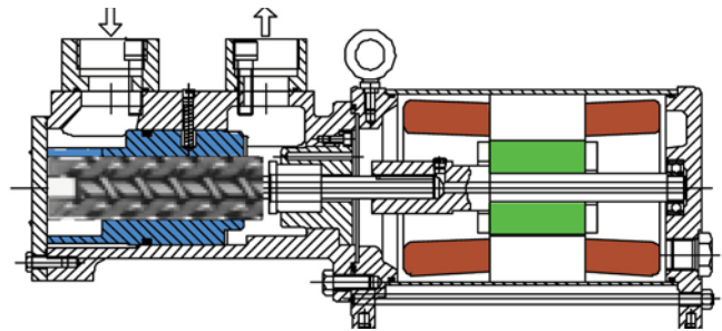
Figure 15: Canned sealless three-screw pump
