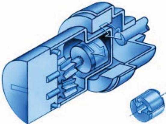
Figure 7: Magnetic drive operation (Courtesy Micropump, Inc.)
